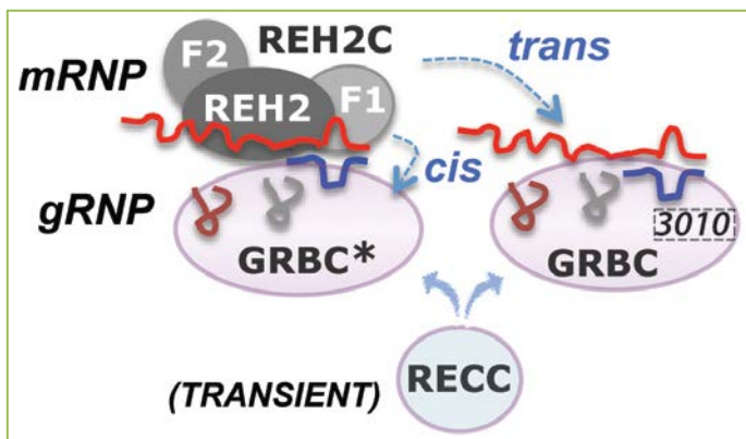
Figure 5. Holo-editosomes include assemblies of auxiliary RNPs and the editing enzyme. This review focuses on the REH2C subcomplex (with its protein subunits indicated as gray ovals). This subcomplex includes the REH2 helicase, two cofactors ( H2 F1 and H2 F2), and all mRNA types involved in editing (pre-edited, partially edited intermediates, and edited). GRBC* and GRBC are variants of another subcomplex that contains gRNAs and several proteins. These gRNA-bound variants (gRNPs) are distinguished by their content of a protein subunit (3010). REH2C binds to GRBC* via stable contacts ( in cis ) and to GRBC via transient contacts ( in trans ). Both types of interaction are via RNA. H2 F1 is proposed to recruit mRNA targets for REH2-catalyzed unwinding of localized secondary structure. The relatively disentangled RNA conformers are more likely to anneal with gRNA or undergo editing at individual sites. The preassembled mRNA-gRNA hybrids in the RNP scaffolds can then be processed by the RECC editing enzyme. Thus, the REH2• H2 F1 system modulates RNA hybrid quality in assembled RNP scaffolds and the ensuing addition of RECC enzyme in complete holo-editosomes. The initiating gRNA (colored blue) hybridizes to the 3' most block in the pre-edited mRNA. The mRNAs are shown in red, and the gRNA transcripts are shown in various colors.
