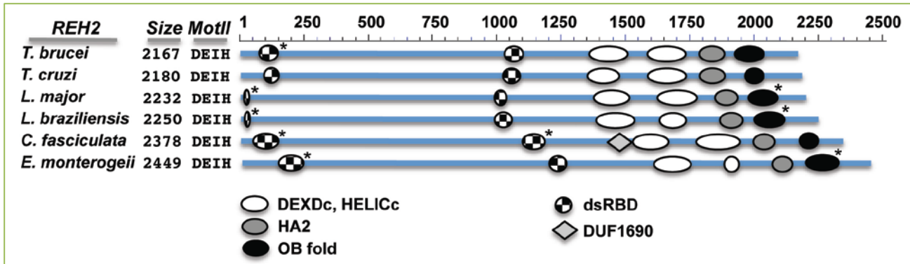
Figure 4. Graphical representation at scale of REH2 orthologs in kinetoplastids. Domain hits were identified in NCBI's interface CD-searches [46] . The CD-search detected a N-terminal dsRBD only in the T. cruzi protein, and an OB-fold in some of the proteins. Three-dimensional structure predictions (*) from the Phyre2 server [47] identified a N-terminal dsRBD and a OB-fold with high confidence in all orthologs. In the Leishmania orthologs, only part of a typical dsRBD was detected. The IDs and sequences of the examined proteins were obtained from the kinetoplastid genome resource TriTrypDB [53] . The species and ID are given as follows: T. cruzi (TcCLB.511003.30 or XP_8160321), L. major (LmjF.34.3230), L. braziliensis (XP_001564561), C. fasciculata (CFAC1_290061800) and E. monterogeii (EMOLV88_340032900). Also indicated are the number of amino acids in each protein and the DEAH family defining residues in motif II.
